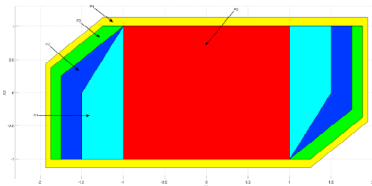
Fig. 5. Sequence of the forward mappings \text{Conv}(\mathcal{P}, A_0\mathcal{P} \oplus A_d\mathcal{P}) leading to a strict superset in 4 iterations
