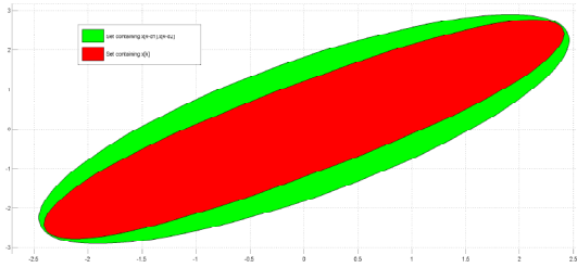
Fig. 1. \mathcal{D} -contractive set for the dDDE (9) with A_0, A_1 in (16)
