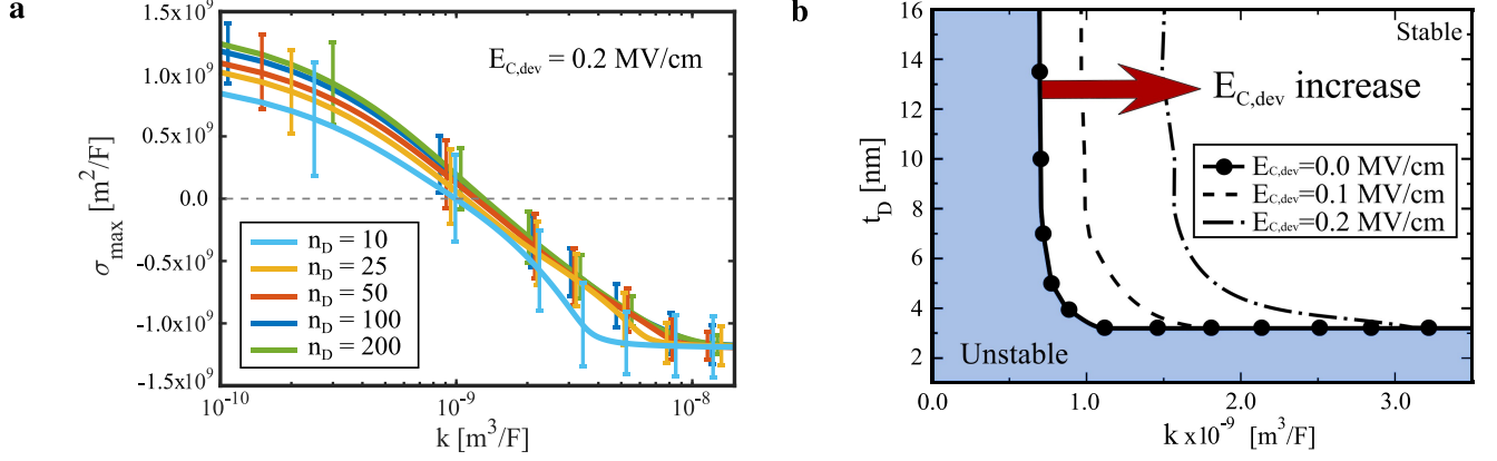
Figure S1: Eigenvalues of the Jacobian matrix and design space for stable NC operation in the presence of statistical dispersion of the anisotropy constants: a. Maximum eigenvalue \sigma_{max} of the Jacobian matrix for a \text{Hf}_{0.5}\text{Zr}_{0.5}\text{O}_2\text{-Ta}_2\text{O}_5 MFIM structure (in the condition of all P_i=0 ) versus the domain wall coupling factor k . Calculations account for a statistical dispersion of \alpha, \beta stemming from a standard deviation E_{C,dev}=0.2 \text{ MV/cm} of the coercive field and correspond to 100 realizations of the MFIM structure. Lines show the \sigma_{max} averaged between the realizations, while the error bar symbols indicate the range between minimum and maximum \sigma_{max} among the different realizations at some k values. Results are shown for different values of the domain number n_D , and all parameters other than n_D, \alpha, \beta are the same as in calculations for t_D=13.5 \text{ nm} in Fig.2(c). b. Regions for stable NC operation for a MFIM structure in the t_D versus k plane and for different standard deviation E_{C,dev} of the coercive field. All parameters other than n_D, \alpha, \beta are the same as in Fig.2 for the case t_D=13.5 \text{ nm}, t_F=11.6 \text{ nm} . Area A=2500 \text{ nm}^2 and n_D=100 .
